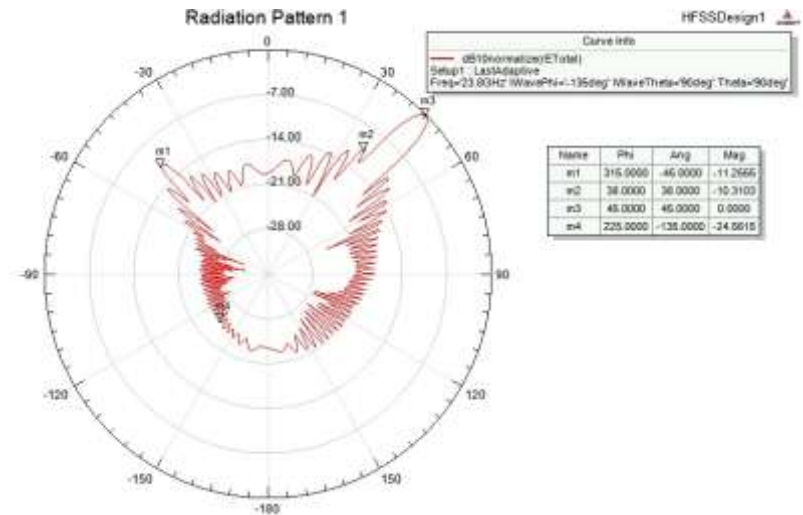
Scattering radiation pattern
