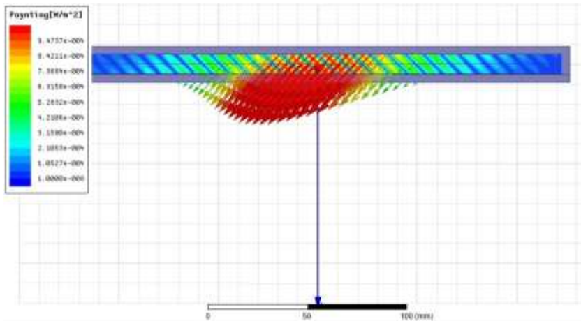
Electric field and power flow through the array plotted
