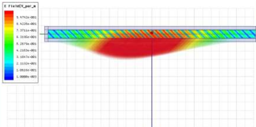
Electric field and power flow through the array
