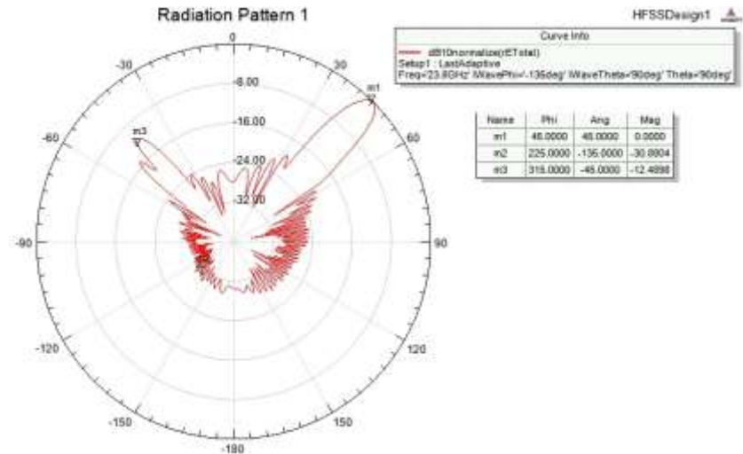
Scattering radiation pattern
