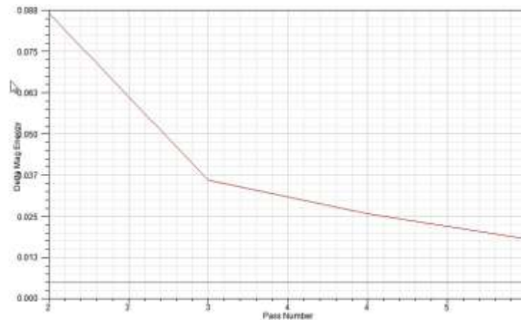
Model convergence
