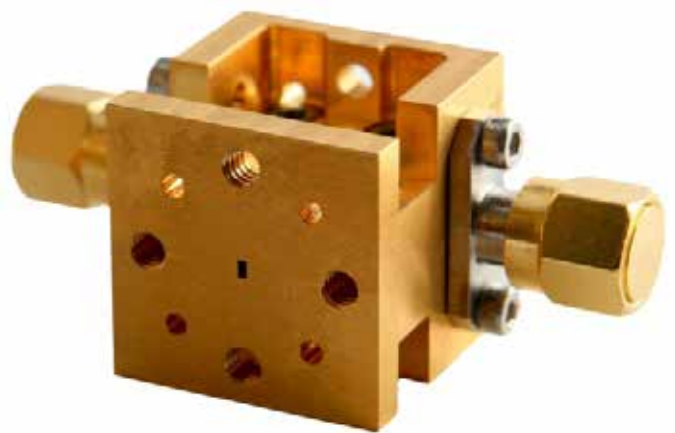
The SHIRM Image Separating Mixer Courtesy STFC-RAL Space
